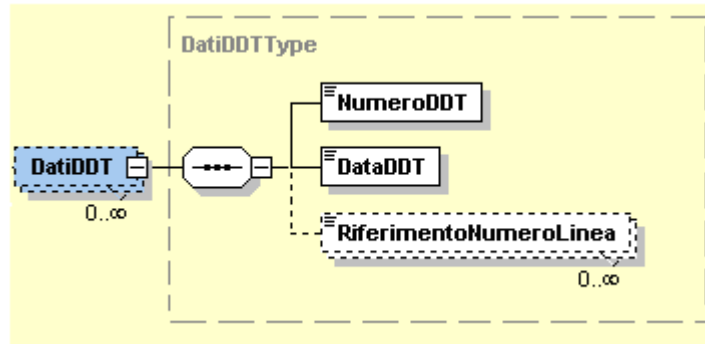
Figure 23: Element DatiDDT
